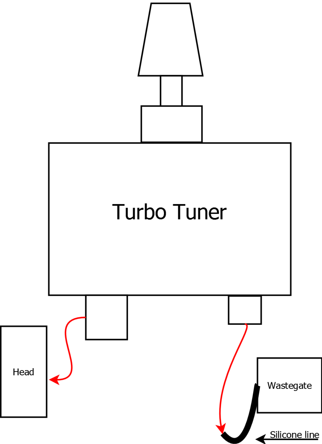
Instal Diagram without AFC LIVE install Package
